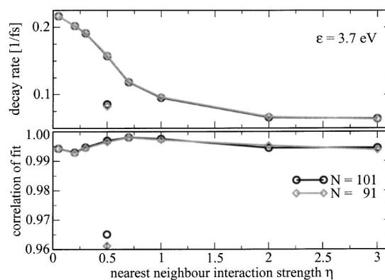
FIG. 6. The decay rates of excited state population which were obtained from an exponential fit of the data shown in Fig. 5 are plotted vs nearest-neighbor interaction strength \eta (upper panel). It decreases for larger values of \eta . The goodness of exponential fit is more or less independent of \eta (lower panel). Two values for the decay rate and the correlation coefficient are plotted for \eta=0.5 eV, once the data of the whole range shown in Fig. 5 and once only values of excited state population up to 25 fs were used in fitting.
