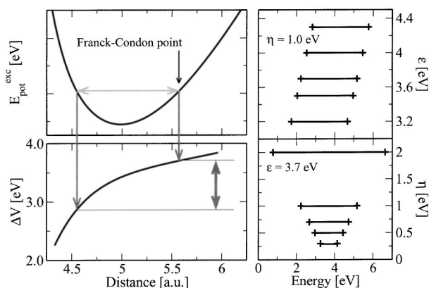
FIG. 3. The range of bath eigenenergies needs to match the difference potential \Delta V for quenching to be efficient (left). It is determined by the bath parameters \varepsilon and \eta (right). The difference potential is fixed by assuming resonant excitation at the Franck–Condon point with a laser energy of 3.7 eV.
