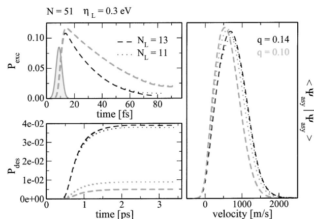
FIG. 13. The dipole strength q determines the lifetime (top left) and it leads to a very slight shift in mean velocity (right). The desorption probability was converged well enough to give an order of magnitude estimation (bottom left).
