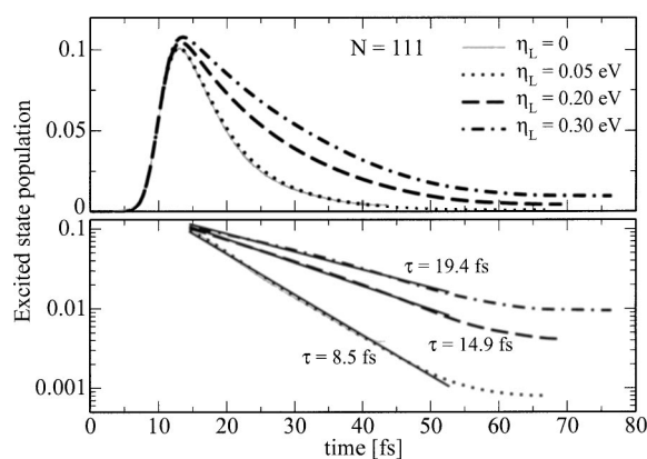
FIG. 8. Increasing the interlayer coupling leads to a slower decay due to faster transport of relaxed population away from the interaction region (parameters as in Fig. 7, but N_L=5 ).
