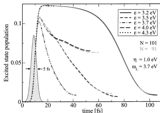
FIG. 4. Dependence of excited state population vs time on the TLS energy \varepsilon : If \varepsilon and therefore the center of the bath energy band is close to the system resonance fixed by the laser energy \omega_L (the dashed curves) the decay of excited state population is exponential, and the choice of \varepsilon determines convergence. If the bath energies are larger than the system resonance (dotted curve), the system cannot give energy to the bath and no decay is observed. For bath energies smaller than the system resonance (solid curve), the wave packet needs to travel to a region where the bath energies match the potential difference before decay can occur (see the text for further explanation). N indicates the number of bath modes.
