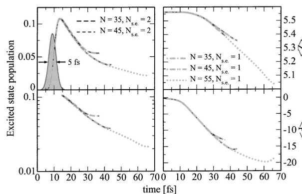
FIG. 1. The excited state population vs time is shown on the left, on a linear (top) and logarithmic scale (bottom). The expectation value of distance (top) and momentum (bottom) of the wave packet on the excited state vs time are shown on the right. Increasing the number of modes N prolongs the convergence time. The number of simultaneously allowed excitations can be restricted to 1 since the black and gray curves are identical. The parameters are \varepsilon=4.0 eV, \eta=2.0 eV, q=0.1 , \omega_L=3.7 eV.
