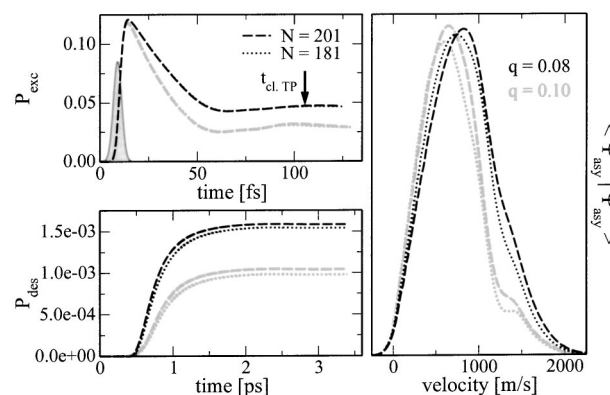
FIG. 14. The same as Fig. 13 ( q varied), but with bath distance switch-off criterion. The velocity distributions have been scaled for comparison.
