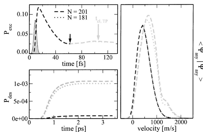
FIG. 10. If the distance of the bath excitation (gray) is used as convergence criterion instead of the population of the system (black), longer convergence times t_S can be obtained (indicated by the black arrow). The time the wave packet spent on the excited state is crucial for both the desorption probability (bottom left) and the shape of the velocity distributions (right, scaled for comparison). The second peak in the velocity distribution can be related to the passage of the classical turning point of the excited state potential (indicated by gray arrow) which has only occurred for the gray curves with N=181 and N=201 . The top left shows the population of the excited state with the pulse (not to scale) indicated (parameters as in the previous figures, but N_L=1 ).
