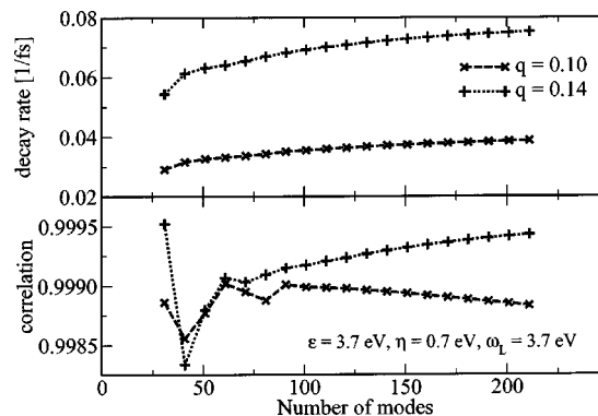
FIG. 2. The excited state decay rate obtained from exponential fit (top) and the correlation coefficient of exponential fit (bottom) are plotted vs the number of bath modes N . The decay rate reaches saturation when increasing N , while the correlation fluctuates in a range close to one.
