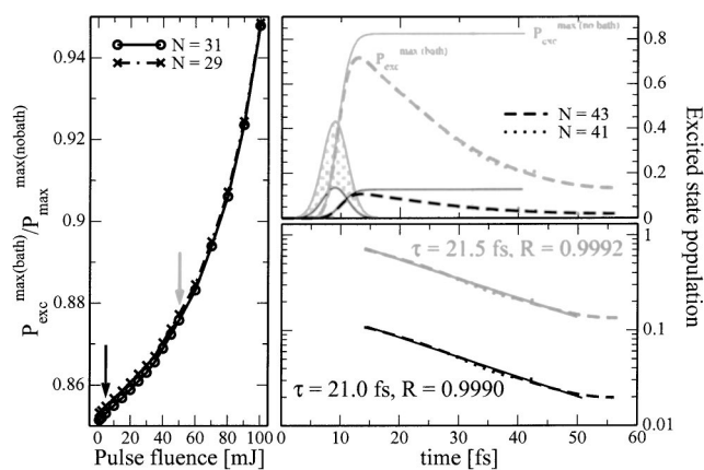
FIG. 15. Dependence of excitation quenching on pulse fluence: energies leading to about 10% excited state population as employed in the other calculations are in the linear regime (indicated by an arrow). The bath parameters are \varepsilon=4 eV, \eta=2 eV with resonant system excitation at \omega_L=3.7 eV and a pulse duration of \tau_{\text{FWHM}}=5 fs. The excited state lifetime is not affected by increasing the pulse energy. The quality of the exponential fit is denoted by the correlation coefficient R .
