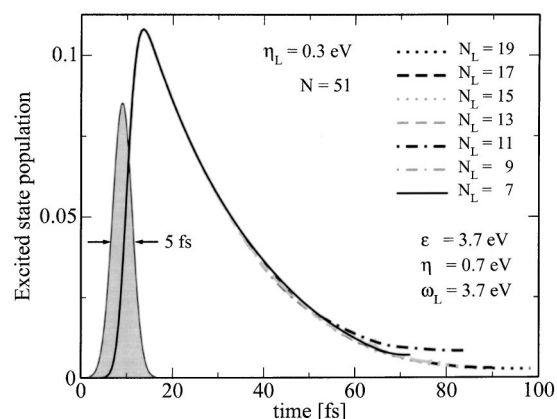
FIG. 7. The population of the excited state vs time. The coupling between electronic states is switched off when recurrences occur, therefore the graph lengths indicate the convergence time.
