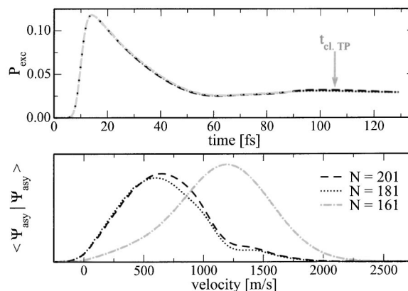
FIG. 11. The gray curves from Fig. 10 are plotted here for increasing number of bath modes N . The appearance of the high velocity peak is related to the passage of the classical turning point, but is independent of the increase in excited state population, i.e., it is not caused by the recurrences in the bath.
